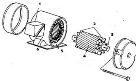
Figure 1. Induction Motor Construction
